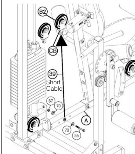
Diagram 2 Pulley Installation
